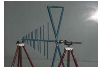
BI-LOG ANTENNA
