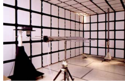
CDC CHAMBER
